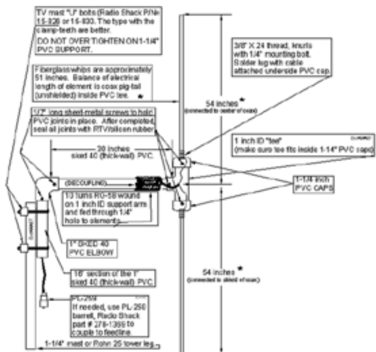
An improved "High-Performance" 6 meter Base-Station Dipole
